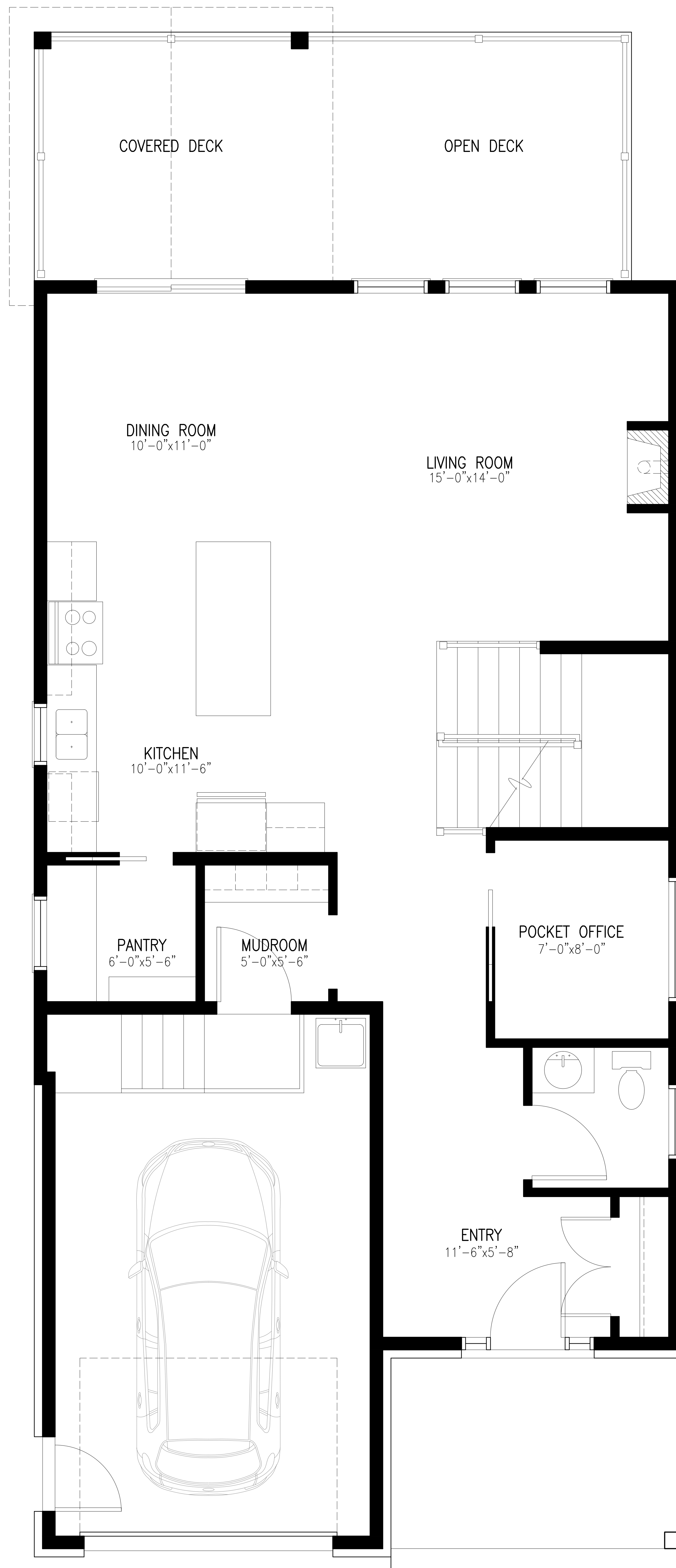
FIRST FLOOR PLAN
